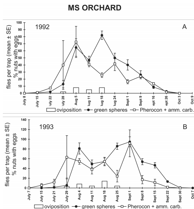
Figure 5 Fly catches on different traps, and oviposition phases recorded in the control of MS orchard in 1992 (A) and 1993 (B).
