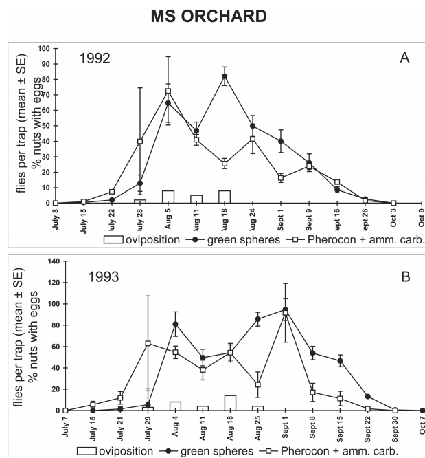
Figure 6 Fly catches on different traps, and oviposition phases recorded in the control of CN in 1992 (A) and 1993 (B).
