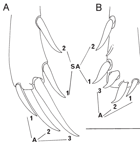
Figure 1 Eneopteroides flavifrons . Inner (A) and outer (B) spurs of hindtibia. Scale = 1 mm. Abbreviations: see material and methods.
