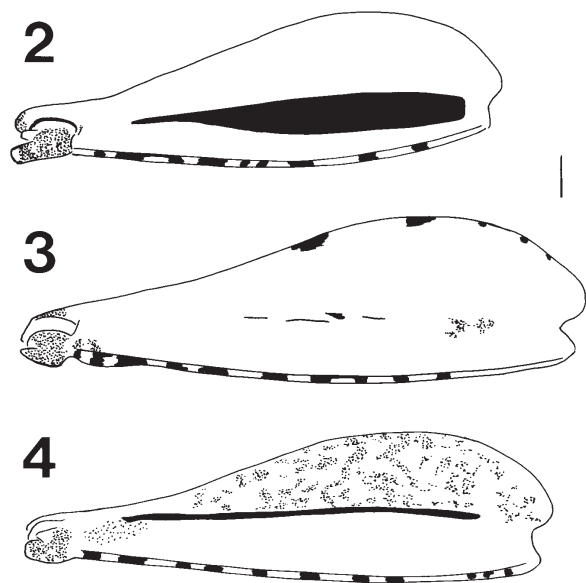
Figures 2-4 Hindfemoral colouration of Eneopteroides species. – 2, E. flavifrons . – 3, E. lorentensis . – 4, E. cordobensis . Scale = 1 mm.
