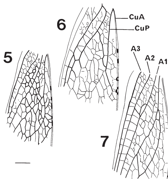
Figures 5-7 Venation of tegminal dorsal field of Eneopteroides species: 5, E. flavifrons . – 6, E. lorentensis . – 7, E. cordobensis . Scale = 1 mm. Abbreviations: see material and methods.
